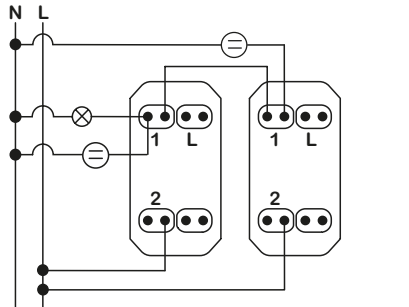
1 module - 2 two-way switches with indication lamp
